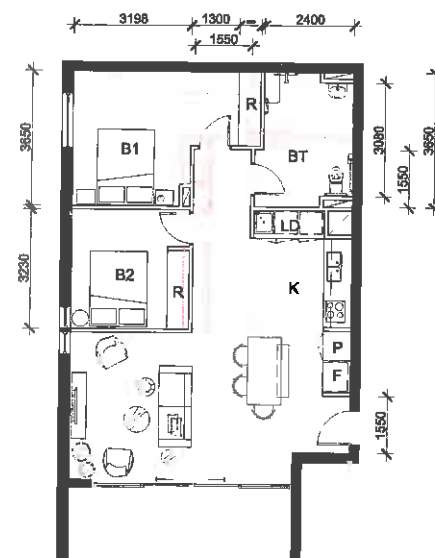
4 Type 3B - 01 POST-ADAPTATION 3B - G.2 3B - 1.2 3B - 2.2 1:100
