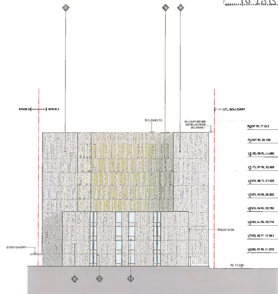
2 SOUTH-WEST ELEVATION BUILDINGS 3A & 3B 1:200
