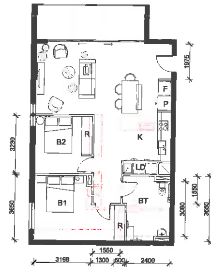
2 Type 3B - 01 POST-ADAPTATION 3B - G.1 3B - 1.1 3B - 2.1 1:100
