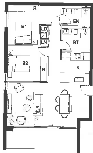
3 Type 3B - 01 PRE-ADAPTATION 3B - G.2 3B - 1.2 3B - 2.2 1:100
