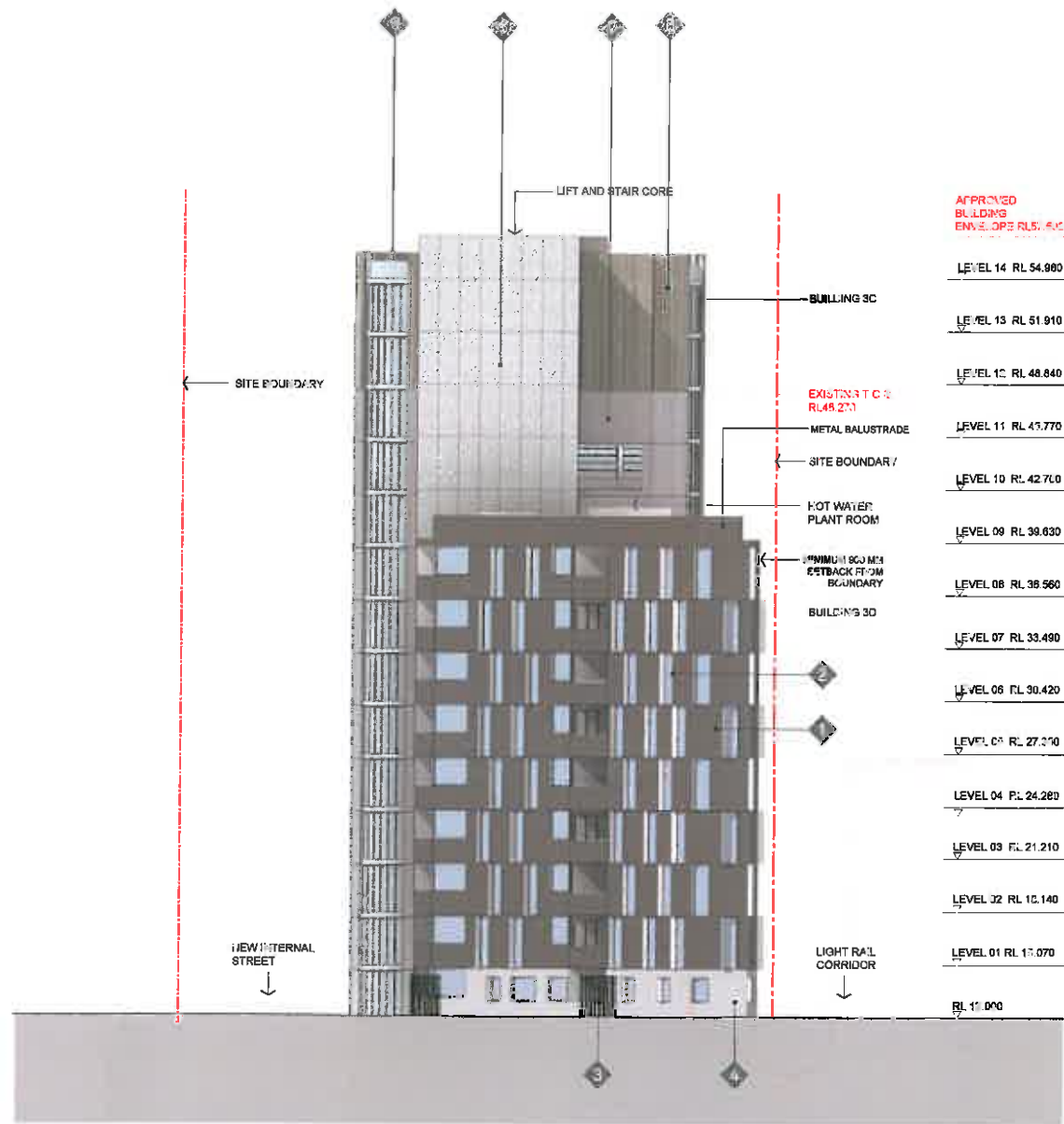
1 SOUTH-WEST ELEVATION BUILDINGS 3C & 3D 1:200
